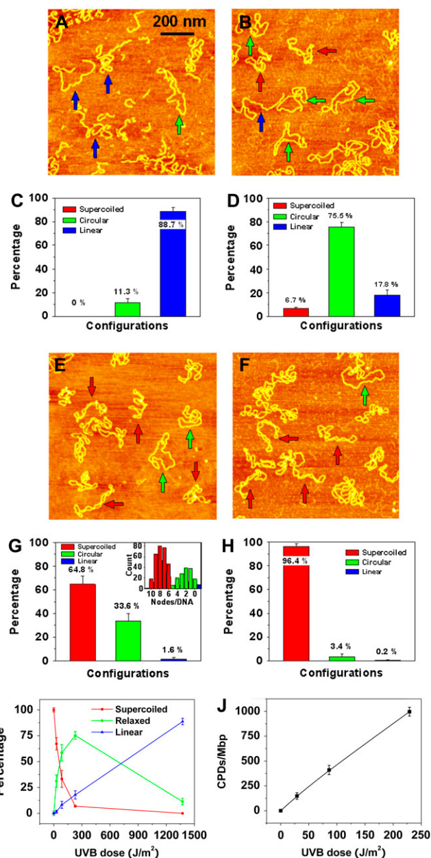
FIGURE 5 AFM images of pUC18 molecules irradiated with different doses of UVB radiation and incubated with T4 Endonuclease V: (A) 1.4 \text{ kJ/m}^2 -irradiated pUC18, (B) 229 \text{ J/m}^2 -irradiated pUC18, (E) 29 \text{ J/m}^2 -irradiated pUC18, and (F) intact pUC18 (control experiment). All scan sizes are 1 \times 1 \mu\text{m}^2 . (C, D, G, H) Histograms of the occurrence of various configurations of pUC18 plasmids determined from AFM images such as these shown in (A, B, E, F). Color code and error bar are the same as in Fig. 2. Each histogram is based on 19–36 AFM images. (I) Percentages of different configurations of irradiated pUC18 as a function of UVB dose. (J) The number of CPDs per million basepairs as a function of UVB dose, supposing the distribution of CPDs follows Poisson.
