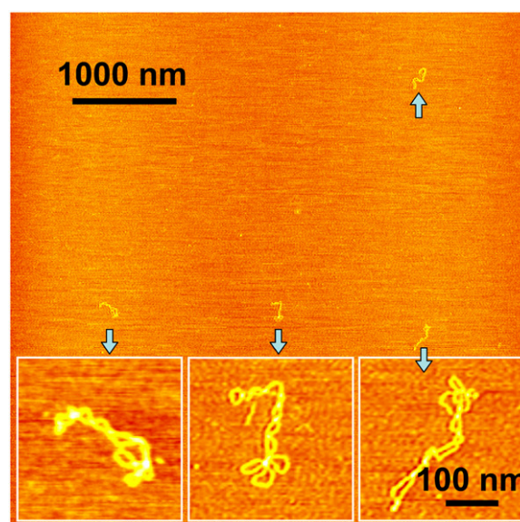
FIGURE 9 AFM image of intact pUC18 plasmids obtained from a sample that contained the total amount of 1 pg of DNA material. Scan size 5 \times 5 \mu m 2 . The inset images obtained at a higher resolution show in detail the supercoiled structure of these plasmids. The scale bar for these inset images is 100 nm. The sample was prepared by spreading 0.1 \mu l of a 10 pg/ \mu l solution of pUC18 on the APS-mica surface and incubating for 3 min. This assay requires extremely small amounts of DNA to evaluate damage.
