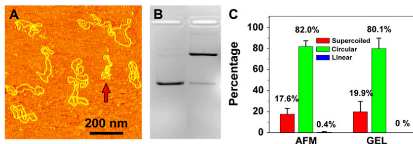
FIGURE 8 (A) AFM images of pUC18 molecules irradiated with 135 J/m 2 UVB radiation and incubated with T4 Endonuclease V. (B) Agarose gel electrophoresis image: lane 1: control, and lane 2: the same sample as in Fig. 8 A. (C) Histograms compare the distributions obtained by AFM and gel electrophoresis as shown in A and B.
