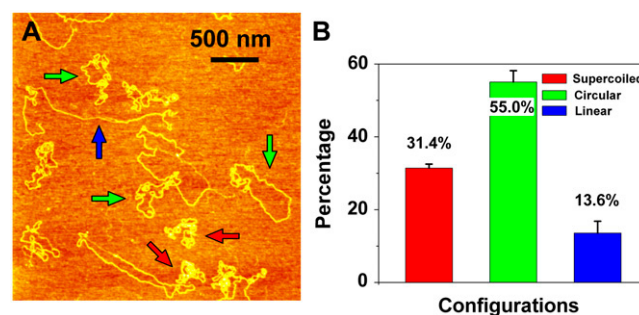
FIGURE 7 Sensitivity of damage detection increases with plasmid size. (A) An AFM image of supercoiled plasmid pNEBR-R1 (10,338 basepairs) irradiated at 29 J/m 2 UVB. Scan size 3 \times 3 \mu\text{m}^2 . (B) Percentages of different configurations of pNEBR-R1 plasmids determined from AFM images such as these shown in A. Color code is the same as in Fig. 2.
