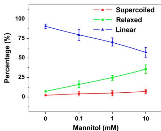
FIGURE 4 Percentage of pUC18 with different structures after 660 \text{ kJ/m}^2 UVB radiation as a function of the concentration of Mannitol.
